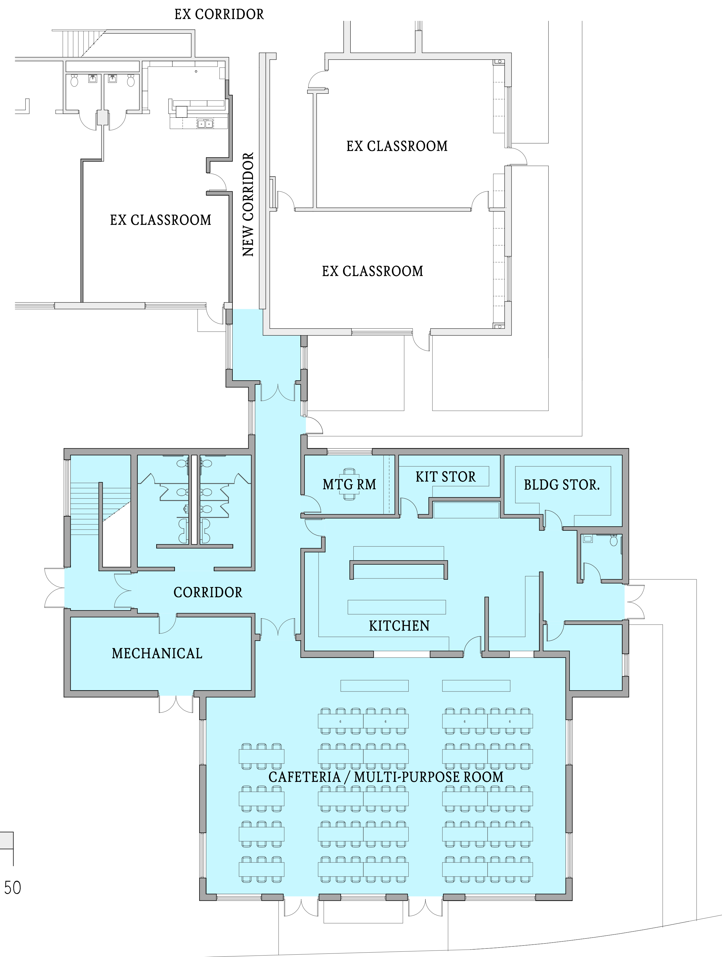
FLOOR PLAN ~ LOWER LEVEL
