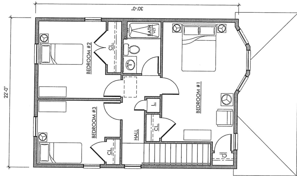
SECOND FLOOR PLAN 672 GSF
