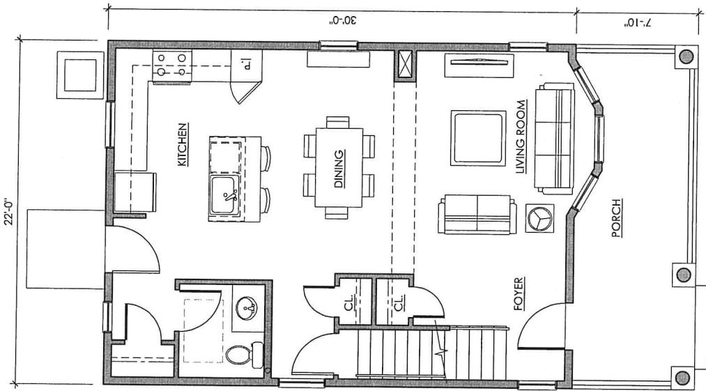
FIRST FLOOR PLAN 672 GSF
